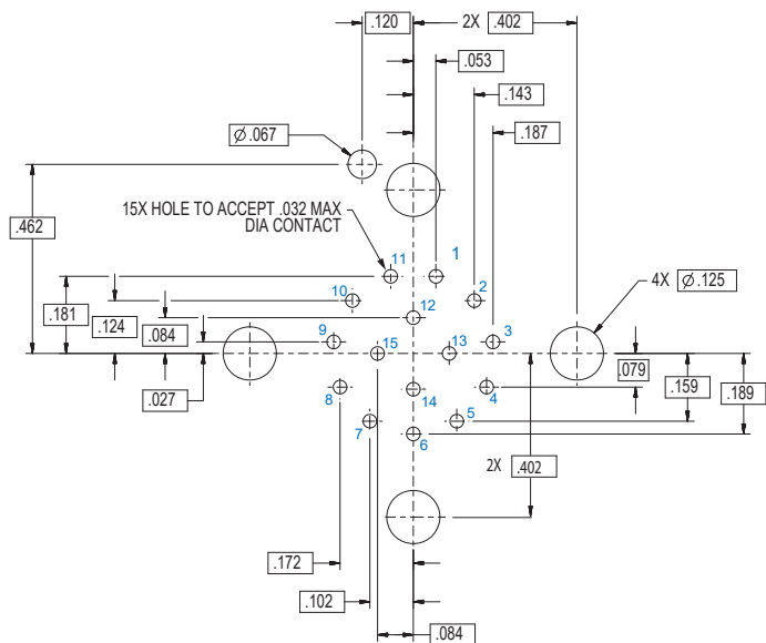
Arrangement No. 12-15 15 #20HD Contacts
