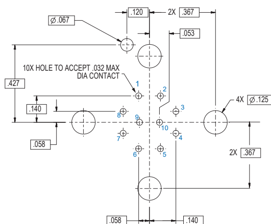
Arrangement No. 11-10 10 #20HD Contacts
