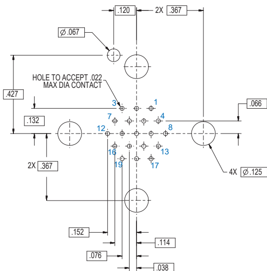
Arrangement No. 11-19 19 #22HD Contacts
