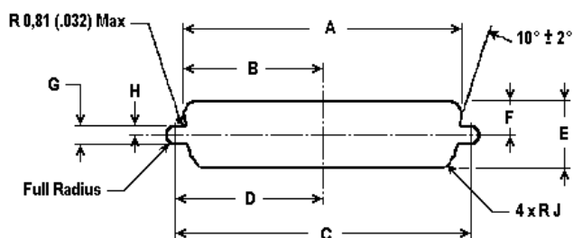
Standard Cutout
